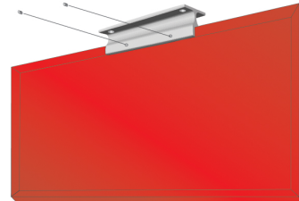
Back, 10-24 X 5/16 Set Screw Location
